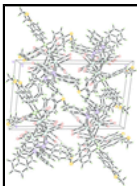
Fig. 2. The crystal packing of the title compound, viewed down the a axis, showing the molecules link into dimers stacking along a axis. Intermolecular hydrogen bonds are shown as dashed lines and solvent molecule have been omitted for clarity.
