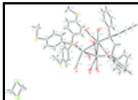
Fig. 1. The molecular structure of the title compound with 50% probability ellipsoids for non-H atoms. Atoms with suffix A are generated by the symmetry operation (1 - x, -y, 1 - z).
